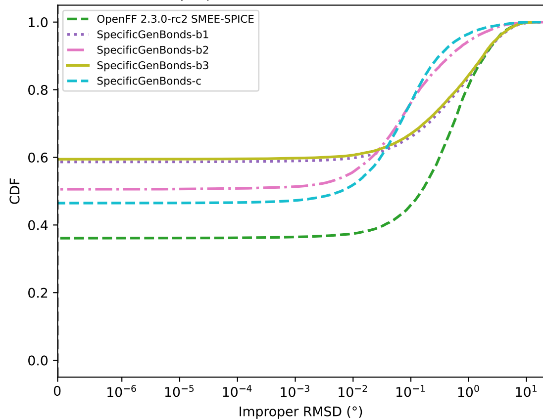
Improper Internal Coordinate RMSD
