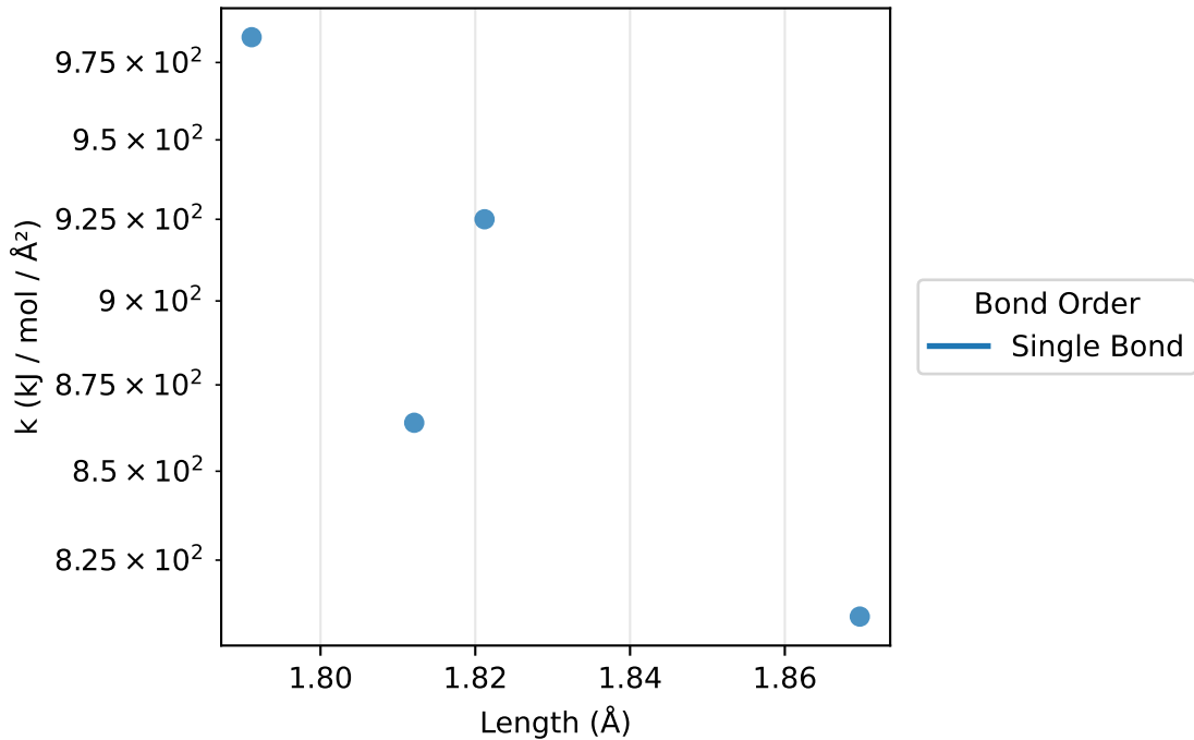
Bonds: k vs length for Br-N (4 params)
