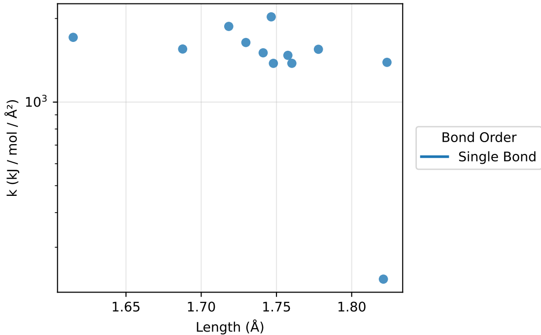
Bonds: k vs length for C-Cl (12 params)
