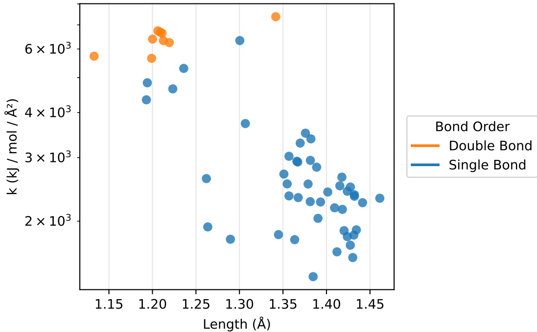
Bonds: k vs length for C-O (55 params)
