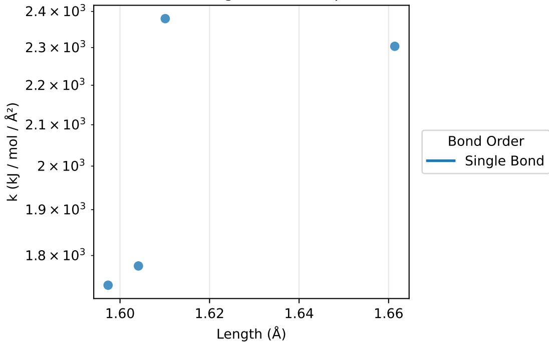
Bonds: k vs length for F-P (4 params)
