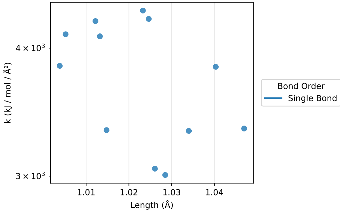
Bonds: k vs length for H-N (12 params)
