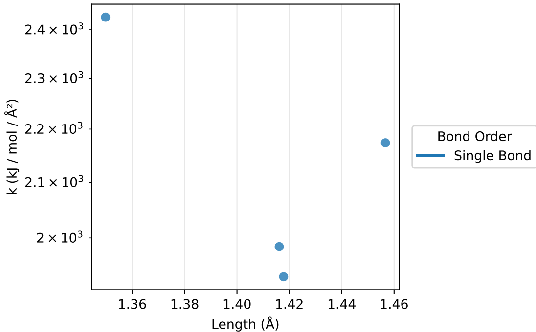
Bonds: k vs length for H-S (4 params)
