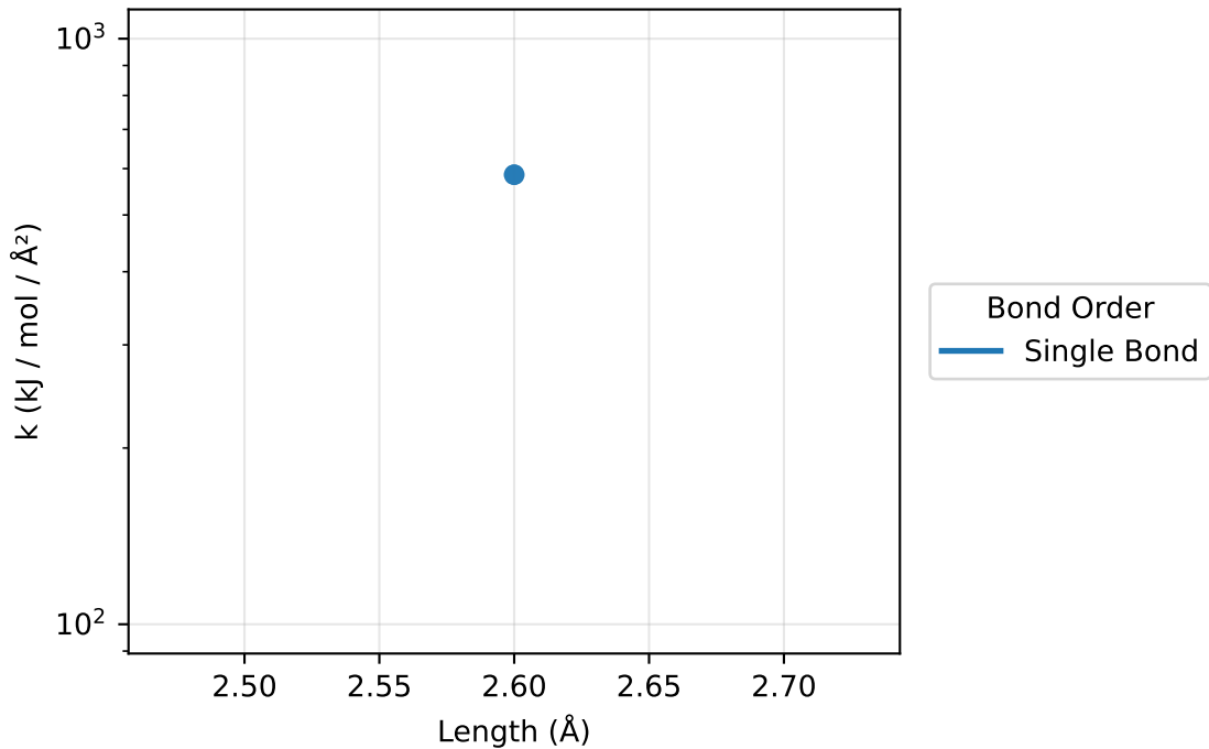
Bonds: k vs length for I-P (2 params)
