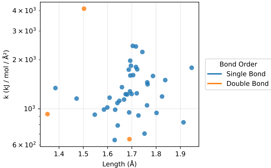
Bonds: k vs length for N-S (43 params)
