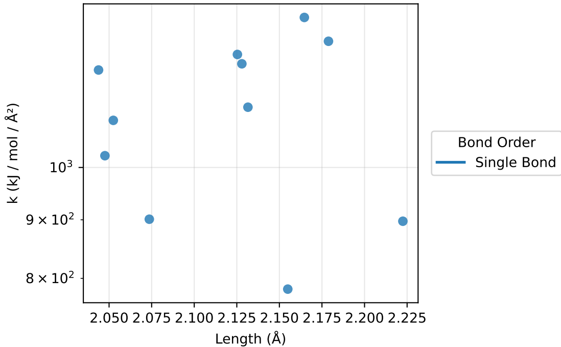
Bonds: k vs length for S-S (11 params)
