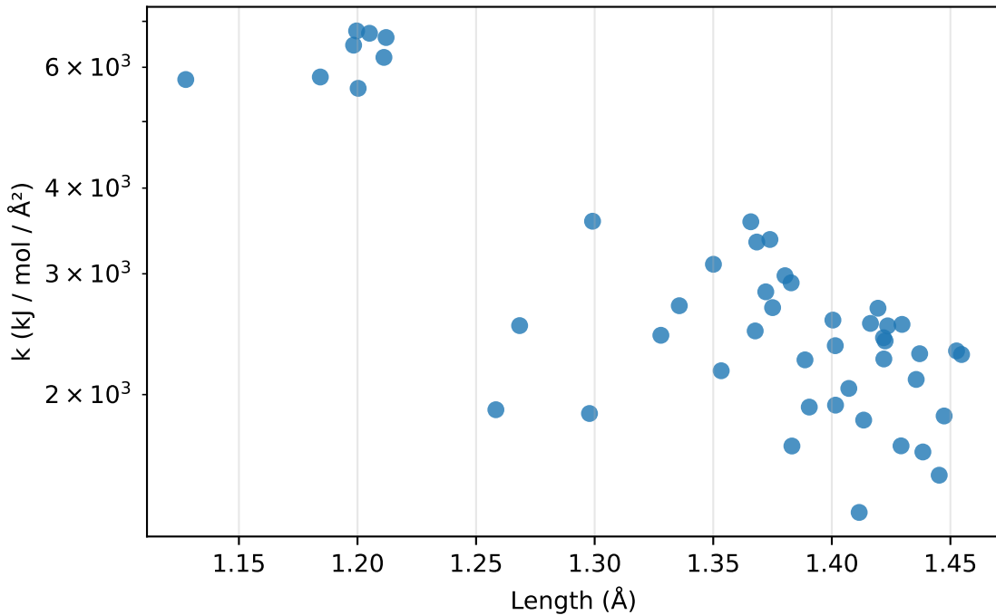
Bonds: k vs length for C-O (48 params)
