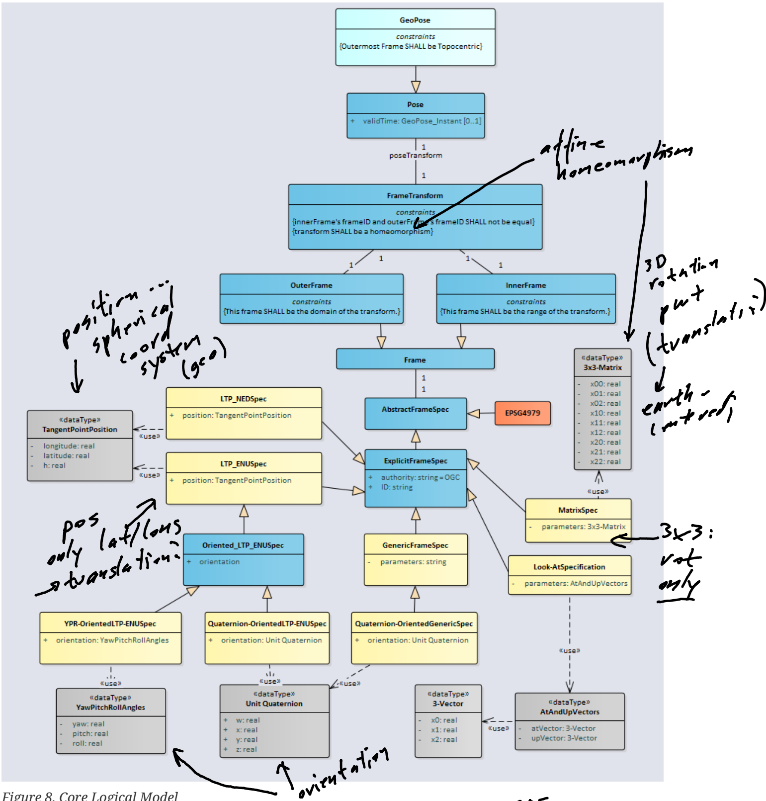
Figure 8. Core Logical Model
