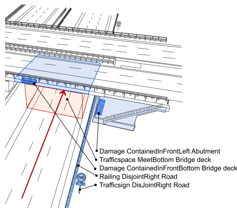
Figure 11 – 3D Topological and Directional relations for 3D objects
