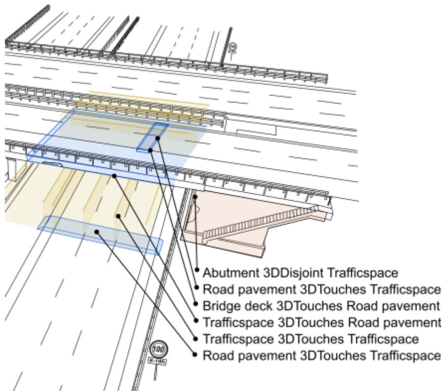
Figure 10 – 3D Topological relations for 3D objects
