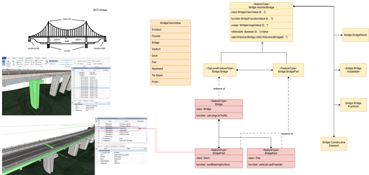
Figure 14 – Model of a bridge where the bridge parts "Pier" and "Deck" contain the geometries of the bridge.
