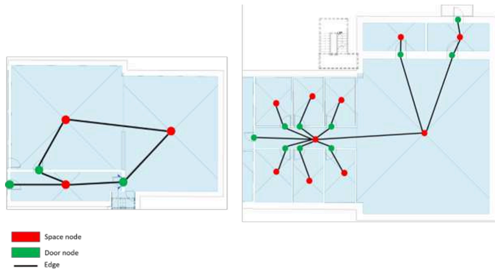
Figure 12 — Space and doors nodes and connecting edges for routing.
