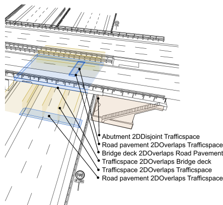
Figure 9 – 2D Topological relations for 3D objects
