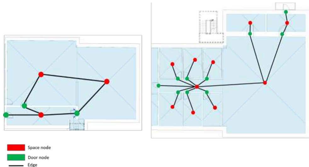
Figure 10 – Space and doors nodes and connecting edges for routing.
