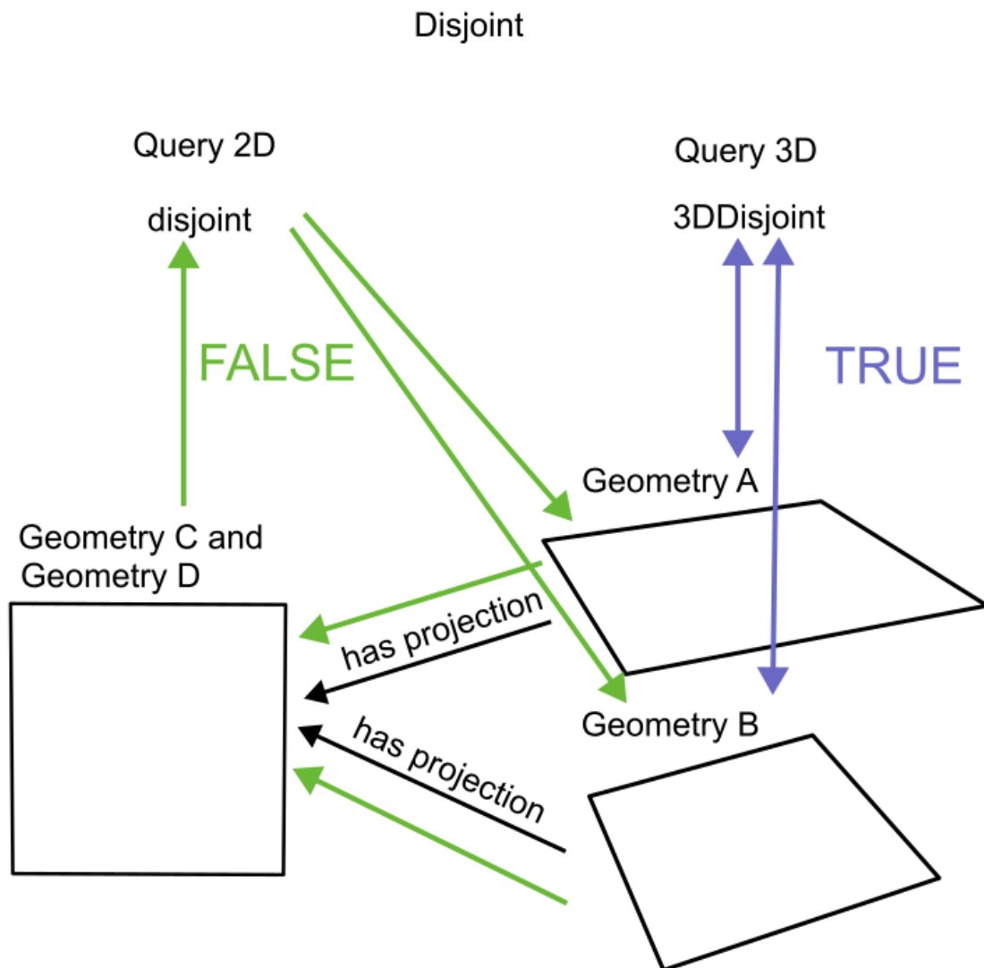
Figure 4 – Disjoint with Query2D and Query3D functions
