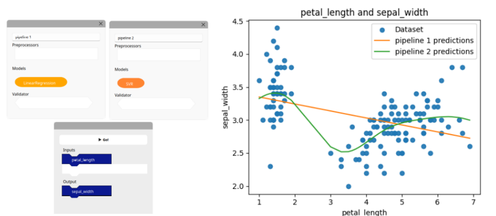
Figure 3: Image showing the model comparison. This would allow novices to understand and visually see the differences between different types of ML models.
