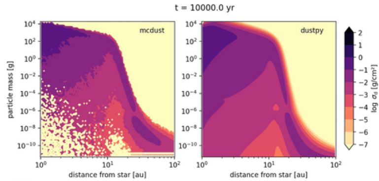
Figure 2: A comparison of the dust surface density \sigma_d as a function of particle mass and distance from the star between mcdust (left) and dusty (right).
