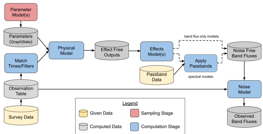
Figure 1: The basic simulation flow for LightCurveLynx
