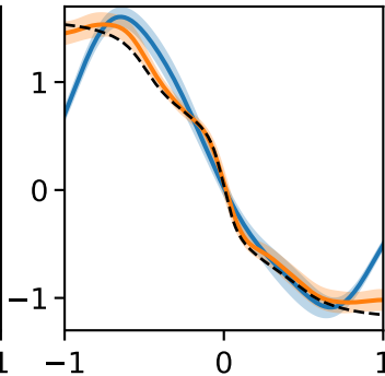
Eigenfunction \psi_1
