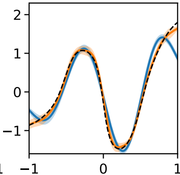
Eigenfunction \psi_3
