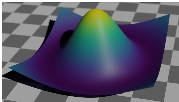
Figure 1: Mesh plot of a Gaussian using a colormap.
