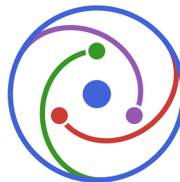
Figure 1: OptimalControl.jl logo.
