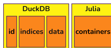
Figure 2: Representation of the storage of indices and JuMP objects
