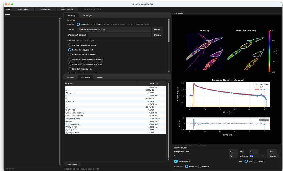
Figure 1: The FLIMKit desktop interface in Single FOV Fit mode. Five freehand regions of interest have been drawn over individual cells and are outlined on both images in the FOV Preview panel, which shows the intensity image and the corresponding per-pixel lifetime map above the summed decay with its reconvolution fit and IRF, and the weighted residuals. The Fit Summary panel lists the recovered tri-exponential parameters ( \tau_1 – \tau_3 with their amplitude fractions), the amplitude- and intensity-weighted mean lifetimes, the fitted background and IRF shift, and reduced \chi^2 (a goodness-of-fit statistic normalised by the degrees of freedom, with values near unity indicating an adequate fit). Per-ROI mean, median, and standard deviation of the fitted lifetime, alongside photon counts, are reported in the Regions table under the ROI Analysis tab. Data are a PicoQuant .ptu acquisition ( 1024 \times 1024 pixels, 1.7 \times 10^6 photons).
