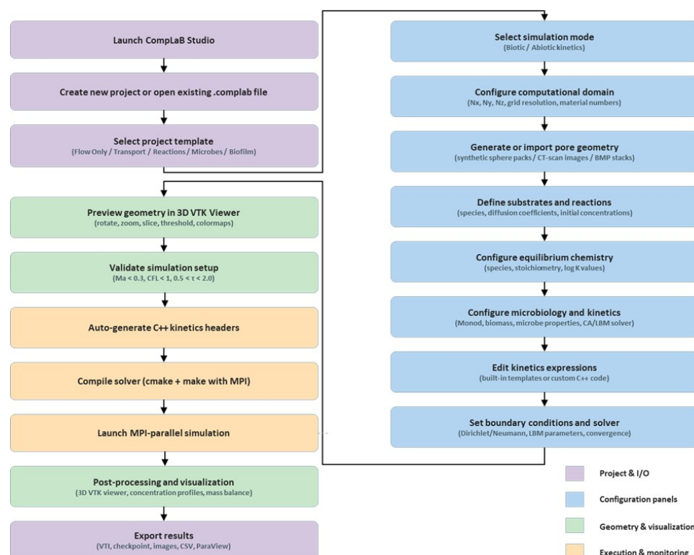
Figure 2: Flowchart of the CompLaB Studio GUI workflow (for more details see Appendix C.14.2).
