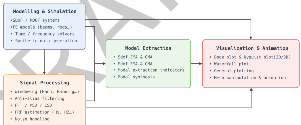
Figure 1: General architecture of StructuralVibration.jl.
