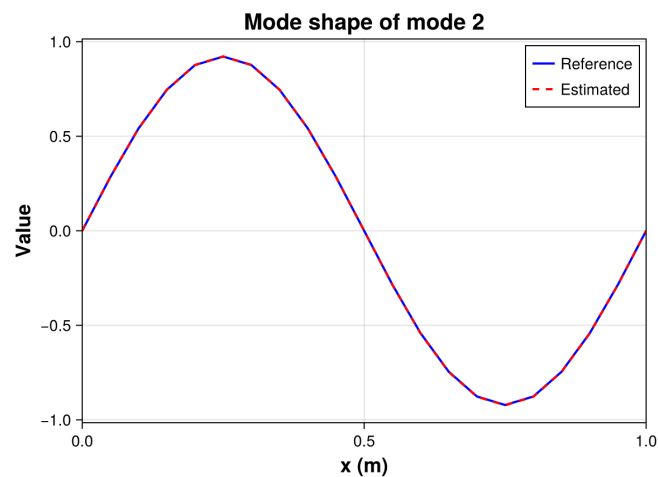
Figure 2: Visualization example - Second mode shape of the beam.
