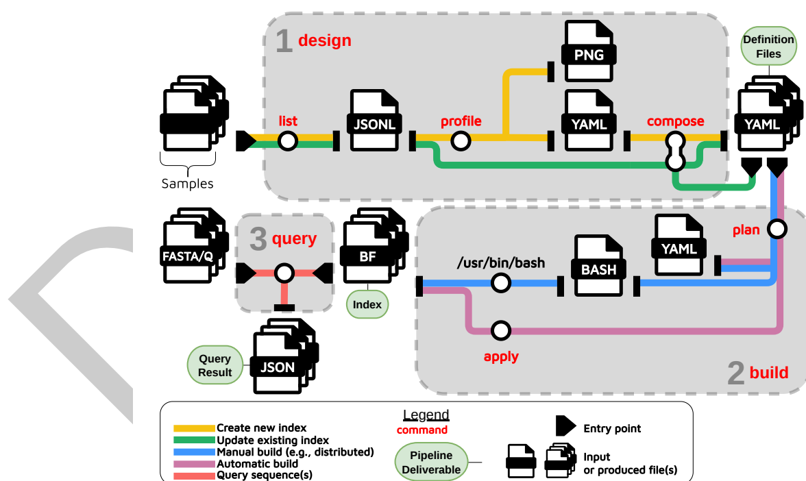
Figure 1: Overview of the kmhelpers workflow
