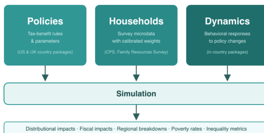
Figure 1: Figure 1: PolicyEngine runtime architecture. Inputs (rules, microdata, and behavioral responses) flow through the simulation pipeline to produce structured outputs.
