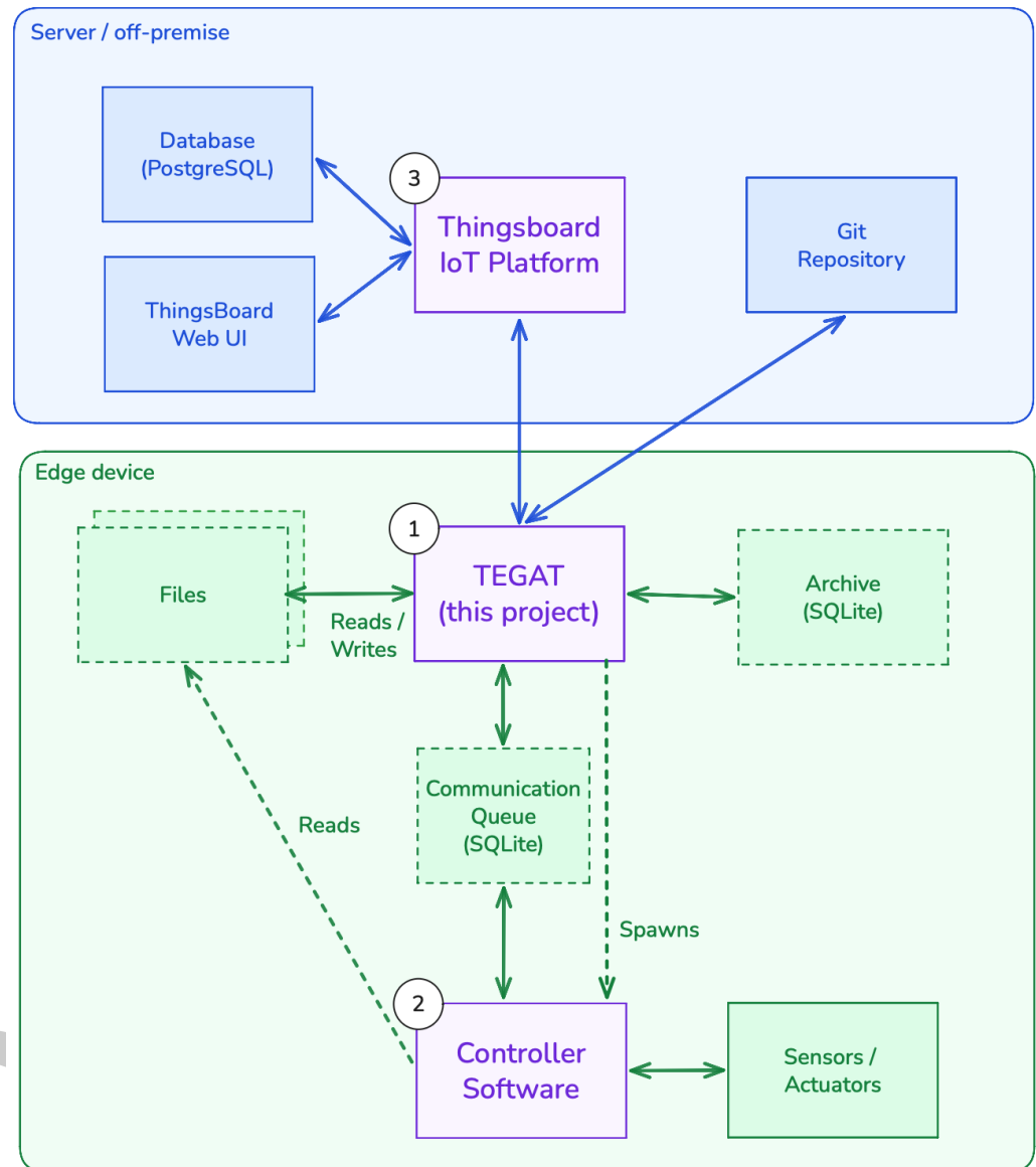
Figure 1: Software architecture for on-device (green) and off-premise (blue) components. Purple boxes show the three main architecture components TEGAT (1), Controller Software (2), and the ThingsBoard IoT Platform (3). Dashed boxes show local files.
