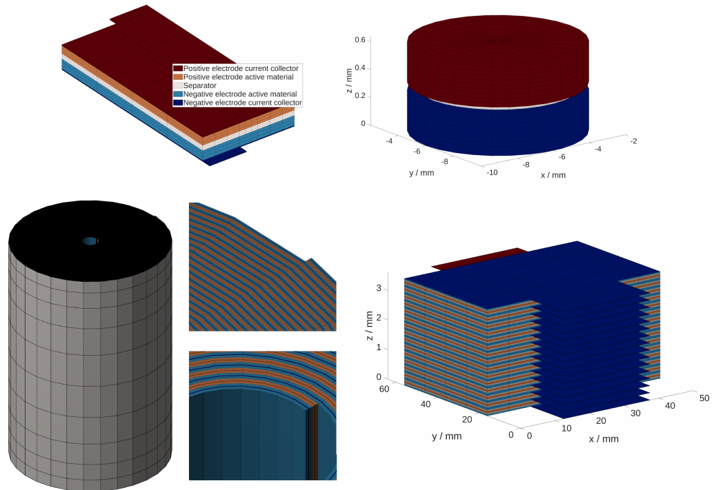
Figure 1: A selection of the parameterized battery geometries available. Clockwise from top left are: A single-layer pouch cell, CR 2016 coin cell, 30-layer pouch cell and jelly roll cylindrical cell.
