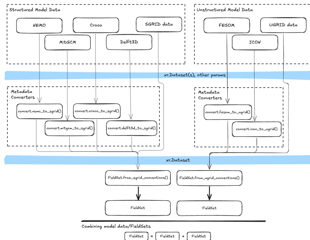
Figure 1: Code path for FieldSet ingestion in v4 of Parcels
