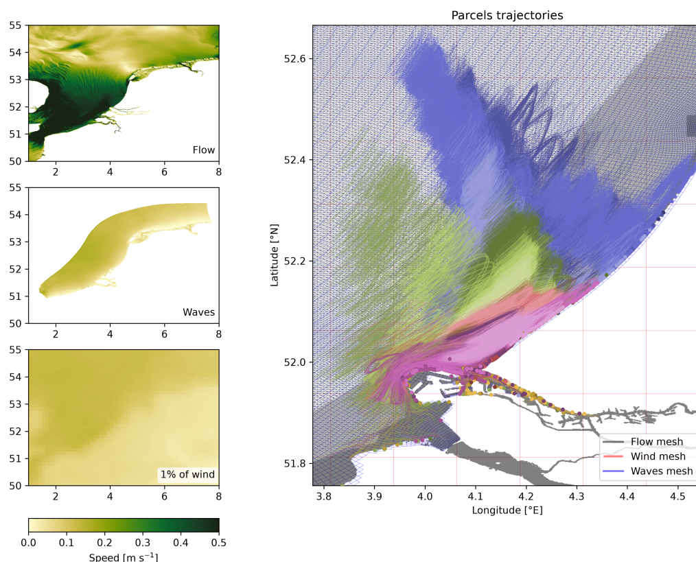
Figure 2: Trajectories of almost 5,000 particles seeded near the port of Rotterdam in The Netherlands. Trajectories are coloured by start date, and final locations of the particles are marked by circles. The mesh of the unstructured flow model (DCSM-FM) is shown in grey, the mesh of the rectilinear Copernicusmarine wind model is shown in red, and the mesh of the curvilinear KNMI wave model is shown in blue.
