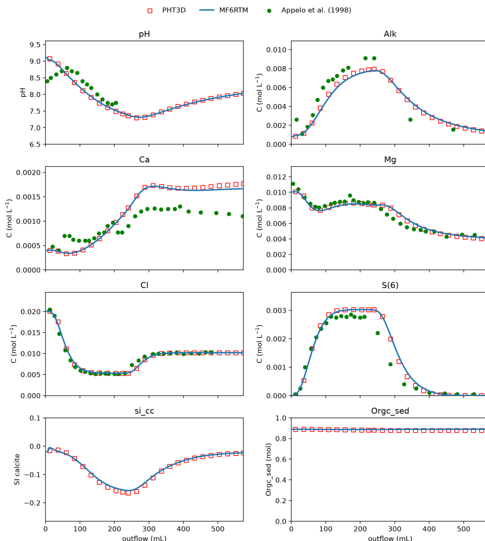
Figure 1: Comparison of effluent concentrations simulated with MF6RTM and PHT3D for Example 5, with the measured data of Appelo et al. (1998).
