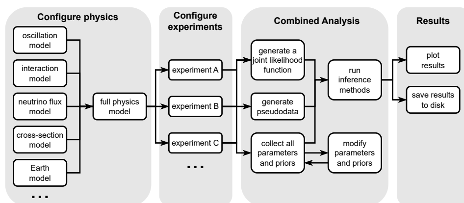
Figure 1: Typical workflow for global analyses of neutrino data with Newtrinos.jl. The layers communicate through two well-defined interfaces: NamedTuples of parameters and priors, and callable functions stored in structs.
