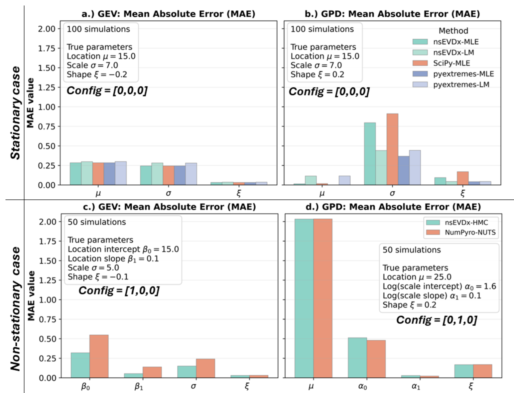
Figure 3: Mean of absolute error in estimating GEV and GPD parameters across the simulations (each using a vector of 500 random values generated using the true parameters) for various methods and Python packages.
