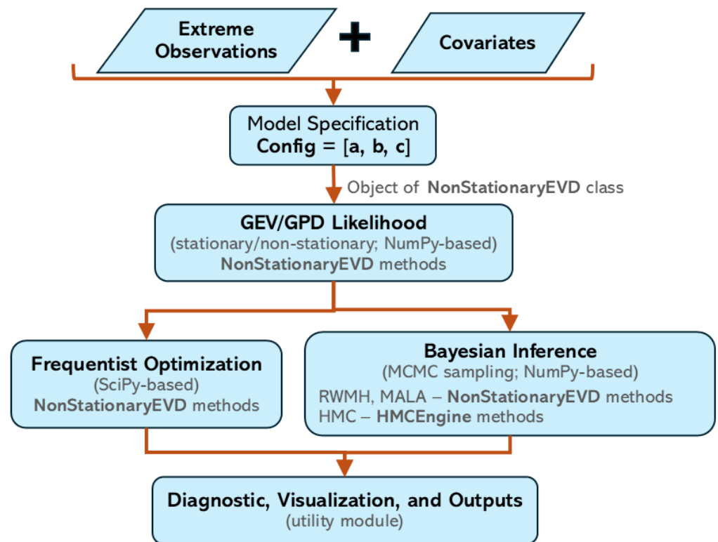
Figure 1: Workflow implemented in nsEVDx for specifying, fitting, and diagnosing stationary and non-stationary GEV and GPD models using frequentist optimization or Bayesian MCMC sampling
