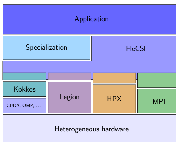
Figure 1: The FleCSI software ecosystem
