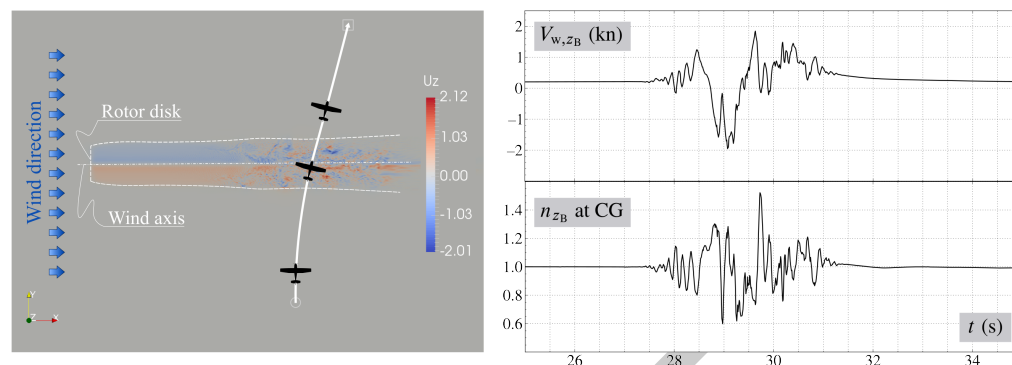
Figure 2: Simulation results adapted from Varriale et al. (2018). Example from a population of simulated scenarios in the presence of CFD calculated wind and turbulence fields. JSBSim's autopilot system has been used to simulate realistic pilot behavior during navigation. (Left) Top view of an airplane flying over a wind-turbine wake. (Right) Time histories of the normal relative-wind component (along z-body axis) induced by the turbine wake, and the normal load factor. Based on these results, preliminary guidelines and recommendations on safe encounter distances have been provided for general aviation aircraft when flying in the proximity of wind farms.
