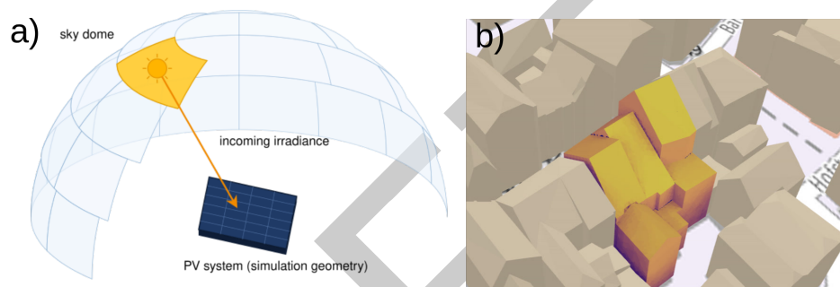
Figure 1: a) Schema of the simulation setup: For each surface of the sky dome and for each triangle of the simulation geometry, it is simulated if an object blocks the incoming irradiance. b) A simulated building with its yearly averaged solar yield, where dark purple represents low yields and light yellow represents high yields. Screenshot taken from (Grosshauser et al., 2024).
