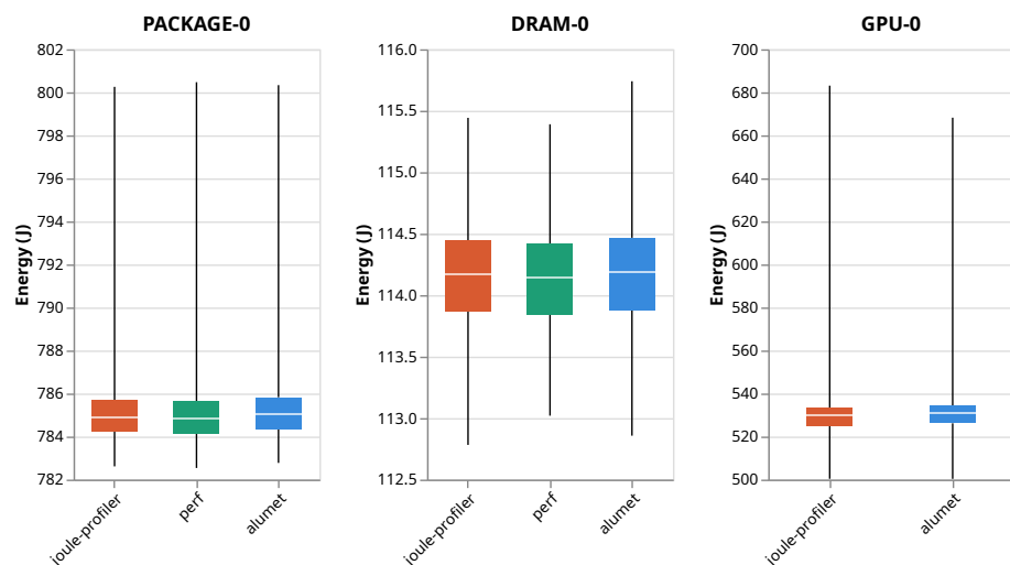
Figure 5: Energy distribution (J) across RAPL domains (DRAM, PACKAGE) and GPU comparing perf, Alument, and Joule Profiler.
