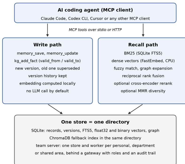
Figure 1: Main parts of total-agent-memory. Agents call MCP tools; writes and searches go to one store per memory area, built around a SQLite database.
