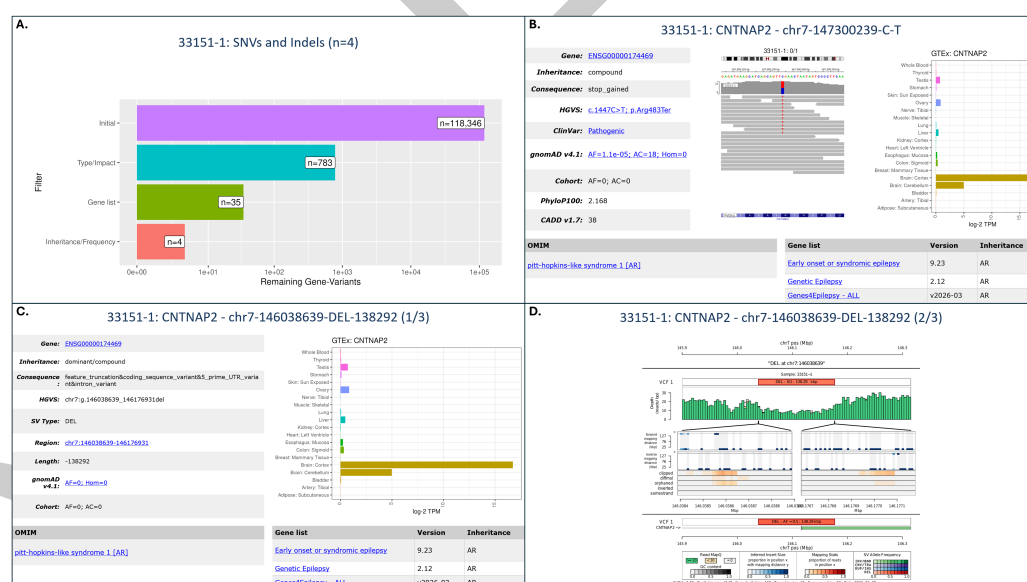
Figure 2: Example nf-cavalier variant PowerPoint output slides for a research participant with compound heterozygous pathogenic variants in CNTNAP2 . A) Summary slide detailing counts after each level of SNV/Indel filtering was applied, resulting in four candidate variants for this example analysis. B) PowerPoint output slide with details on a stop-gain variant known to be pathogenic in ClinVar. Blue text represents hyperlinks to external resources. C) PowerPoint output slide detailing a 138 kb deletion affecting CNTNAP2 . D) nf-cavalier PowerPoint slide embedding an SVPV plot of the structural variant for inspection and QC. This case has been published in Munro et al. (Munro et al., 2026).
