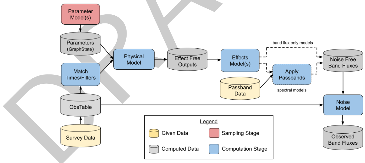
Figure 1: The basic simulation flow for LightCurveLynx
