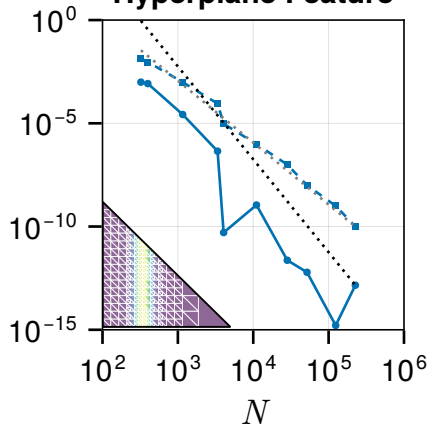
Hyperplane Feature
