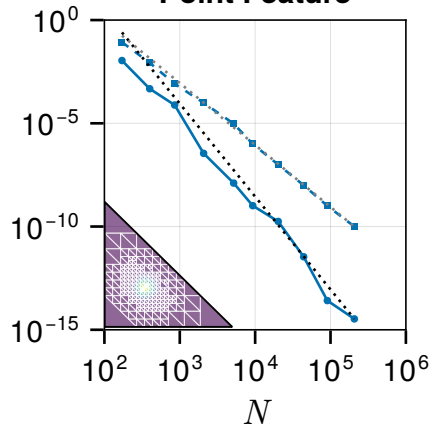
Point Feature
