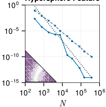
Hypersphere Feature
