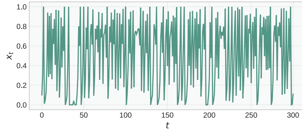
Logistic Map
