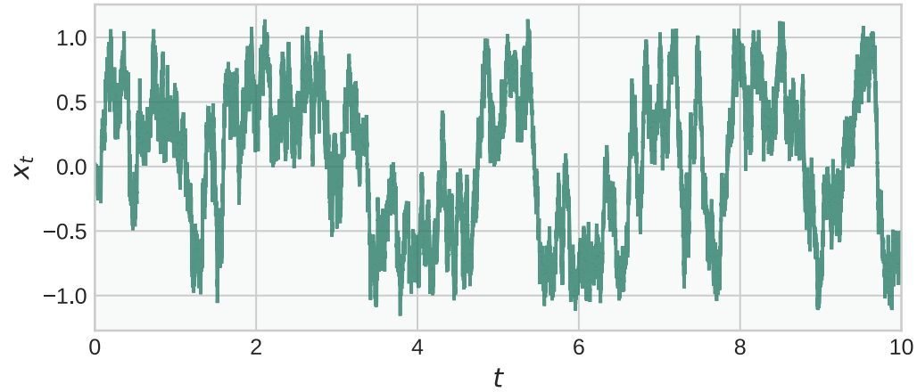
Prinz Potential Trajectory (Metastable States)
