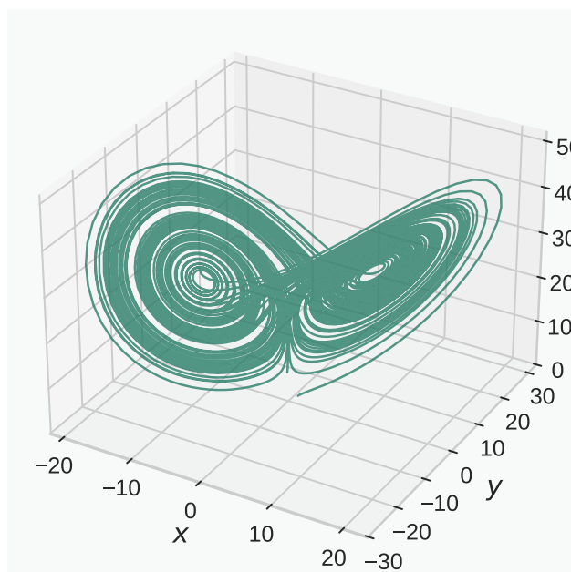
Lorenz-63 Attractor
