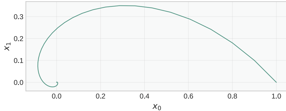
Linear System Trajectory (Spiral Convergence)
