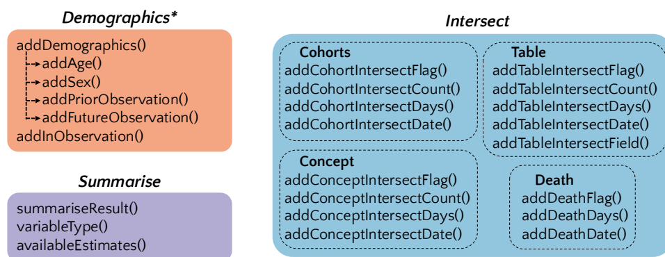
Figure 1: PatientProfiles functions blocks. Note that each demographic function has its own analogous query function to only add a query to the data, e.g. addAge() and addAgeQuery() .
