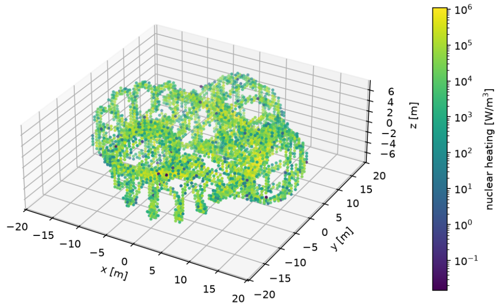
Figure 2: Nuclear heating in the coils of Figure 1 at 3.1 GW fusion power, computed with OpenMC on the geometry built by cadrum (logarithmic color scale).
