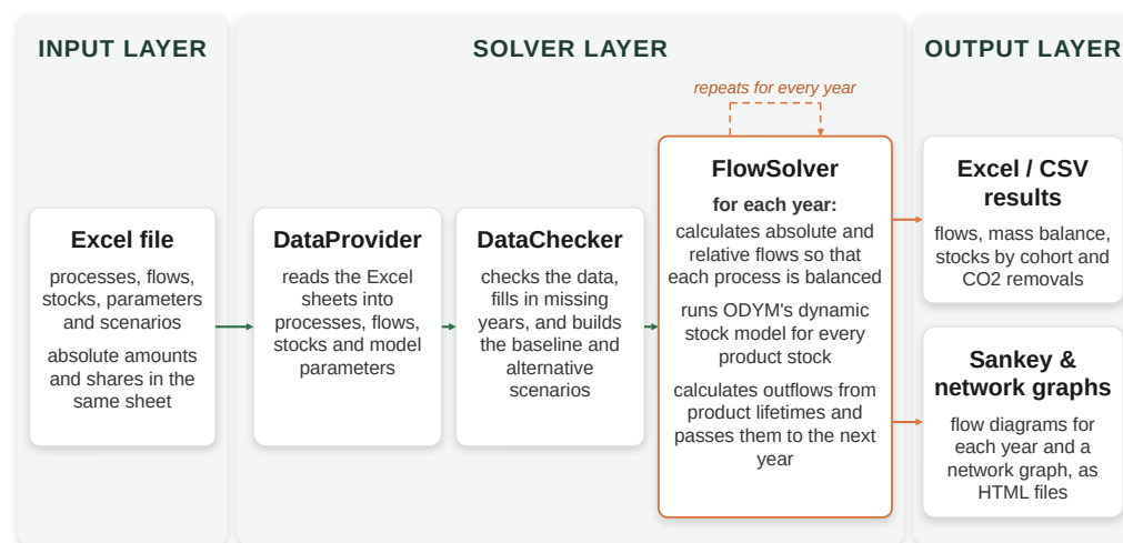
Figure 1: The three layers of an aiphoria run, from the Excel input to the results.
