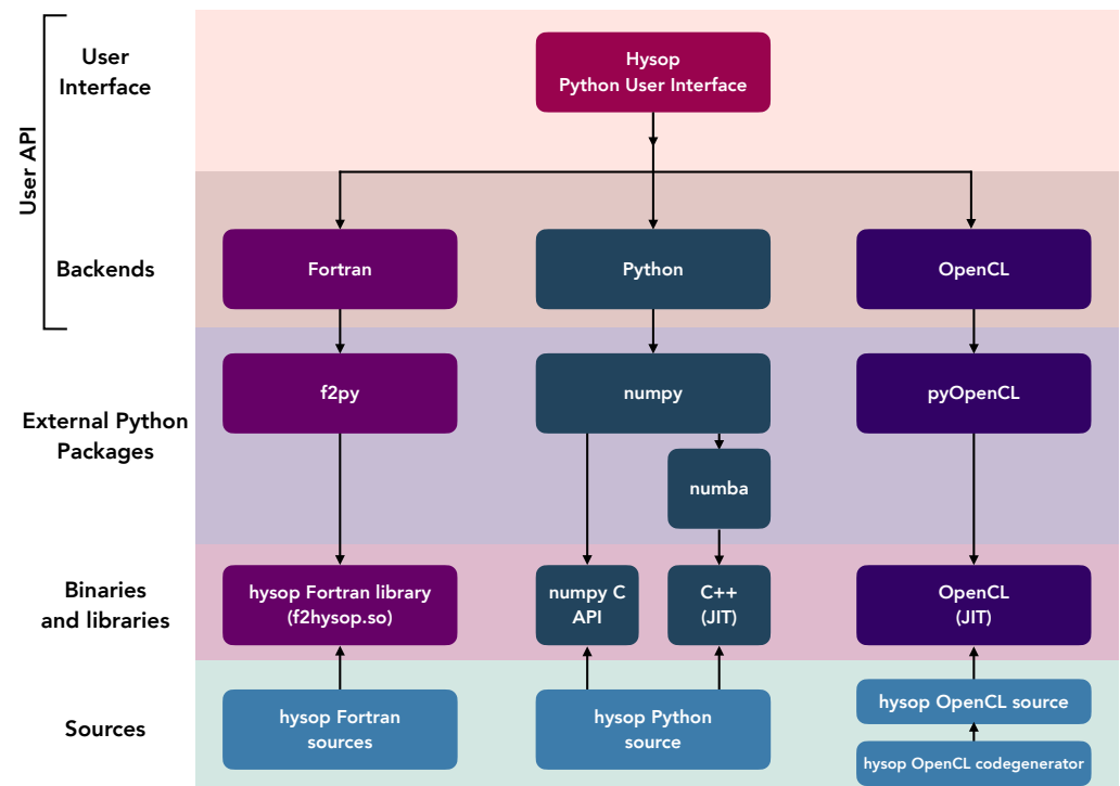
Figure 2: Computing backends in HySoP
