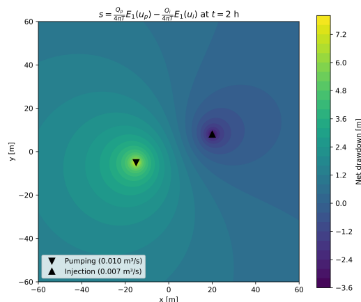
Figure 4: Spatial drawdown field at t = 2 h for the pumping-injection dipole. The pumping well (▼) and injection well (▲) produce an asymmetric drawdown pattern.
