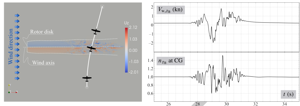
An example from a population of flight simulation scenarios in the presence of CFD calculated wind and turbulence fields. JSBSim's autopilot system has been used to simulate realistic pilot behavior during navigation. (Left) Top view of an airplane flying over a wind-turbine wake. (Right) Time histories of the normal relative-wind component (along z-body axis) induced by the turbine wake, and the normal load factor.
