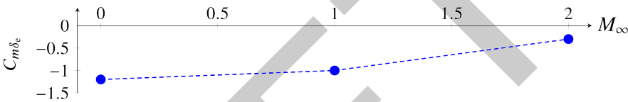
Figure 1: Pitching control power coefficient as a tabulated function of Mach number. See <table> element in the above snippet.
