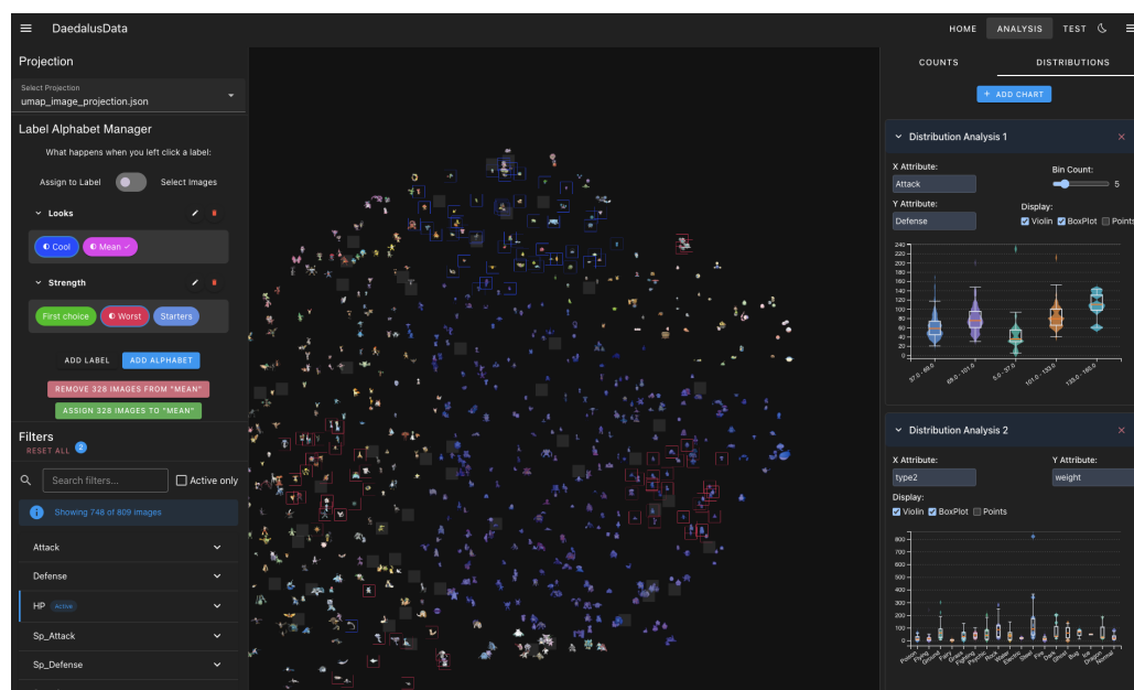
Figure 1: The analysis view on the 809-image demo dataset. Left: projection selector, two label alphabets and metadata filters. Center: the projection, with labeled images framed in the color of their label. Right: violin and box plots of metadata attributes.
