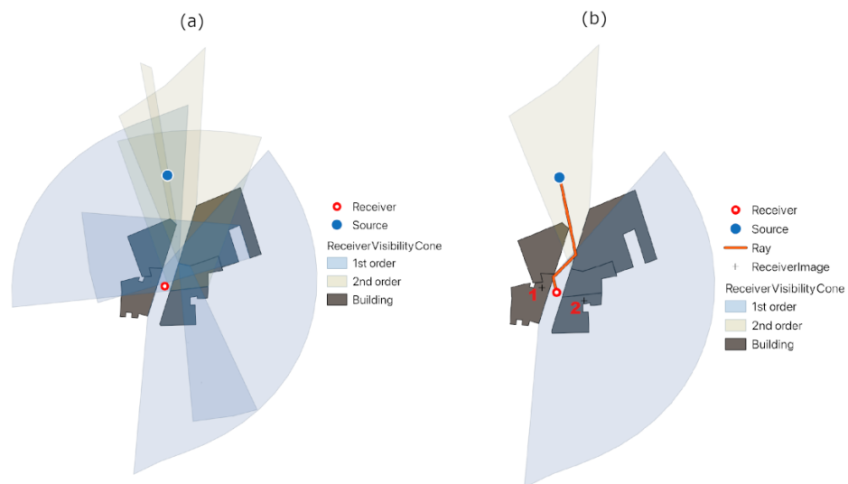
Figure 4: Receiver view cones. (a) All receiver view cones that intersect the source point and its parent order view cone. (b) The only valid reflection is second order: it bounces first on the blue then on the yellow receiver view cone.
