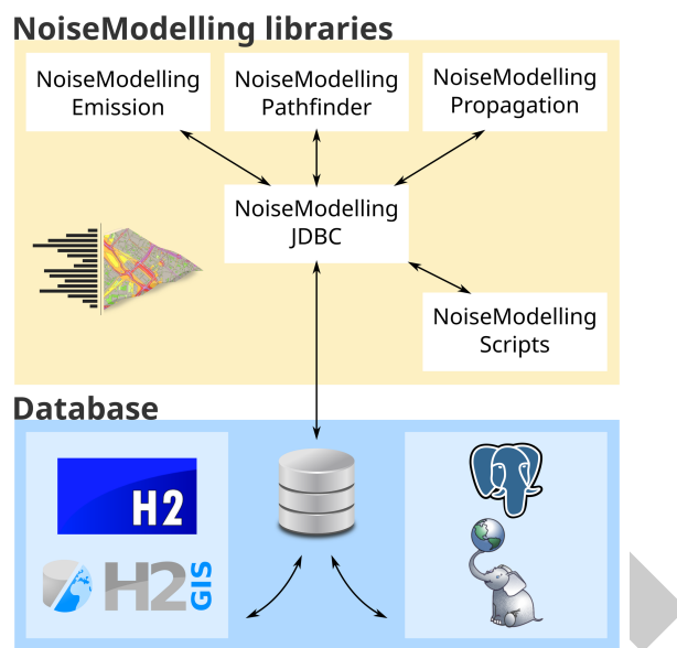
Figure 2: The NoiseModelling Architecture.
